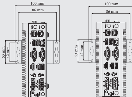
Dimension of the iEP-7030E Series with Wall Mounting Bracket Installed
